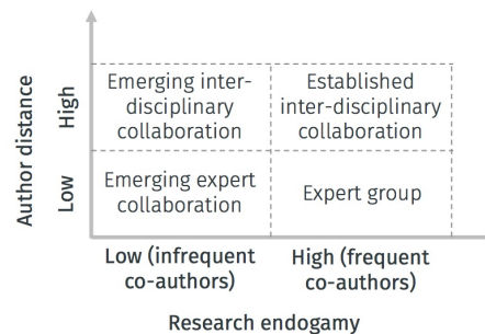
Figure 1: Types of research collaboration based on semantic distance of authors, and their collaboration frequency.
