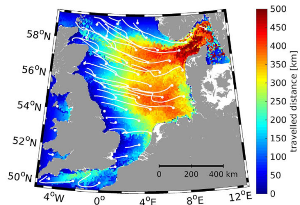
Fig. 6. Displacement of particles from their seeding position over 30 days of integration of the Lagrangian model (19.02.-21.03.2018). The color scale represents the respective distance (lengths of great circle arcs) between the release location and the final position. Exemplary trajectories (64 out of 11,969 in total) are also shown in white. White circles indicate the initial positions. These particles have the properties of the GPS drifter. (For interpretation of the references to color in this figure legend, the reader is referred to the Web version of this article.)
