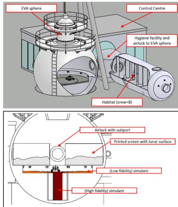
Figure 17: COMEX HYDROSPHERE Lunar Surface Simulator
