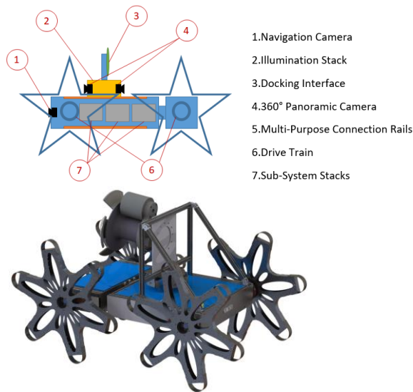
Figure 8: TRACTOR general system layout and bread-board design
