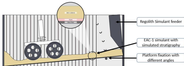
Figure 15: Current design of the wheel testbed
