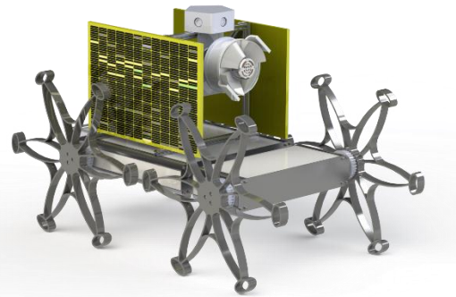
Figure 9: Artist's view of the TRACTOR flight model with potential solar array mountings
