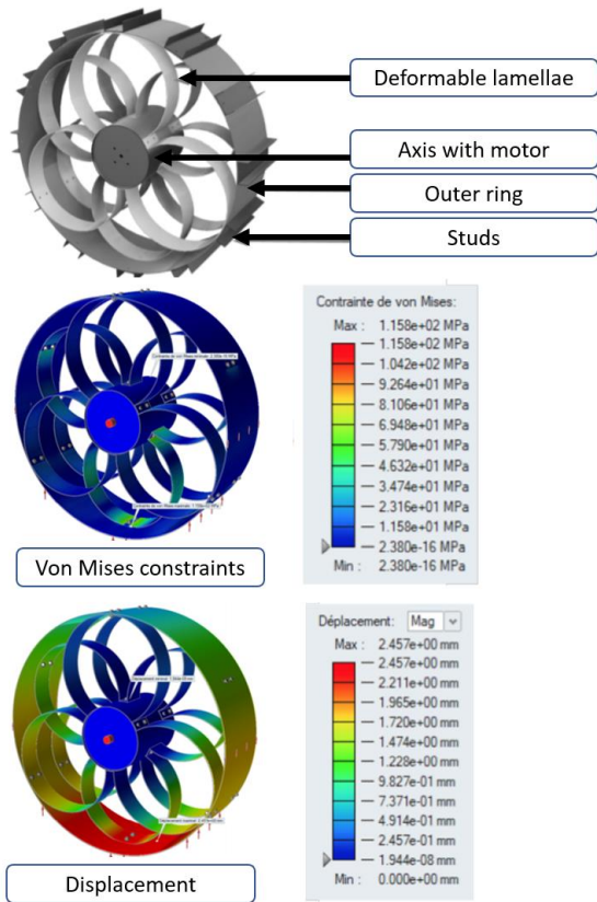
Figure 14: (top) Design of the deformable wheels of WAIN. (middle) Von Mises constraint analysis and (bottom) deformation.
