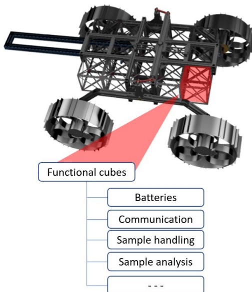
Figure 11: Modular chassis of the WAIN
