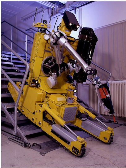
Fig. 7. KHG's robot capable of climbing stairs.
