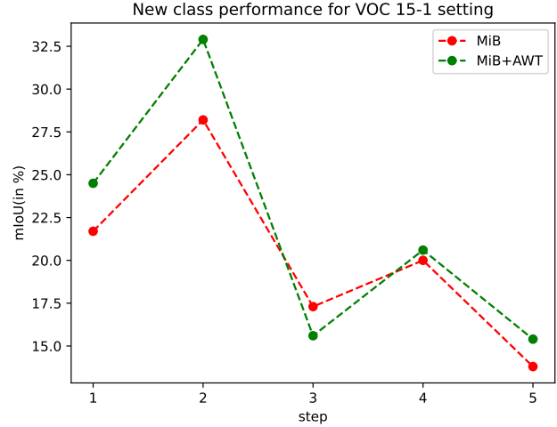
(a) VOC 15-1 setting
