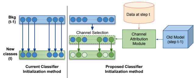
Figure 1: Comparison of classifier initialization methods. Classifier initialization was previously found to be crucial to obtain good plasticity [7, 8, 18, 49, 54] of an incremental learner. However, the method did not address the background shift . Previous methods (left) copy all filter weights from previous background (bkg) to initialize new classes , our attribution-based weight selection (right) explicitly addresses the semantic background shift by selecting only the relevant weights for the classification of new classes . This allows us to combine the plasticity of the previous initialization method with a further reduction of catastrophic forgetting.
