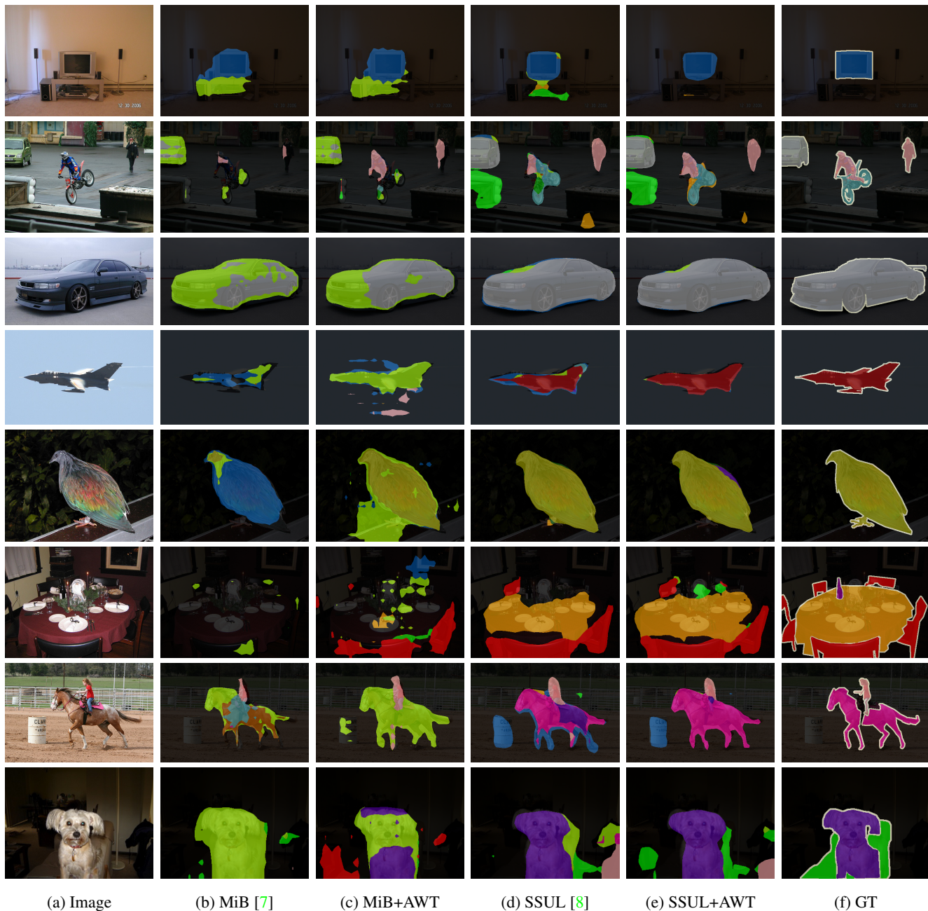
Figure 8: Visualization of predictions using MiB, MiB+AWT, SSUL and SSUL+AWT in 10-1 setting on test images of Pascal-VOC 2012.
