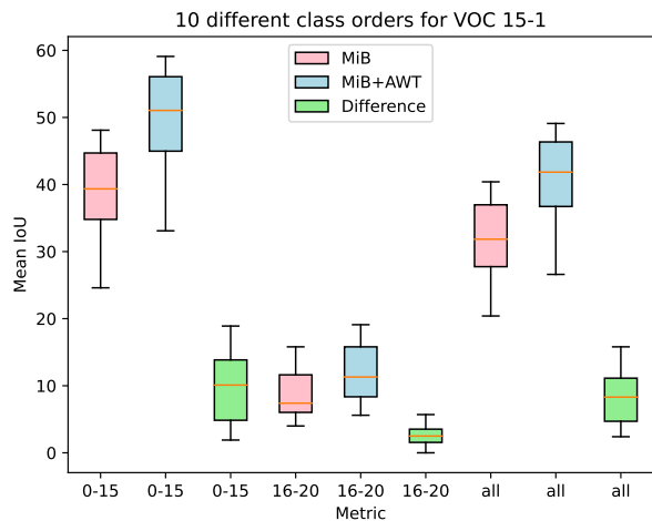
Figure 4: Boxplots of the mIoU of initial, new, and all classes for 10 random class orders.
