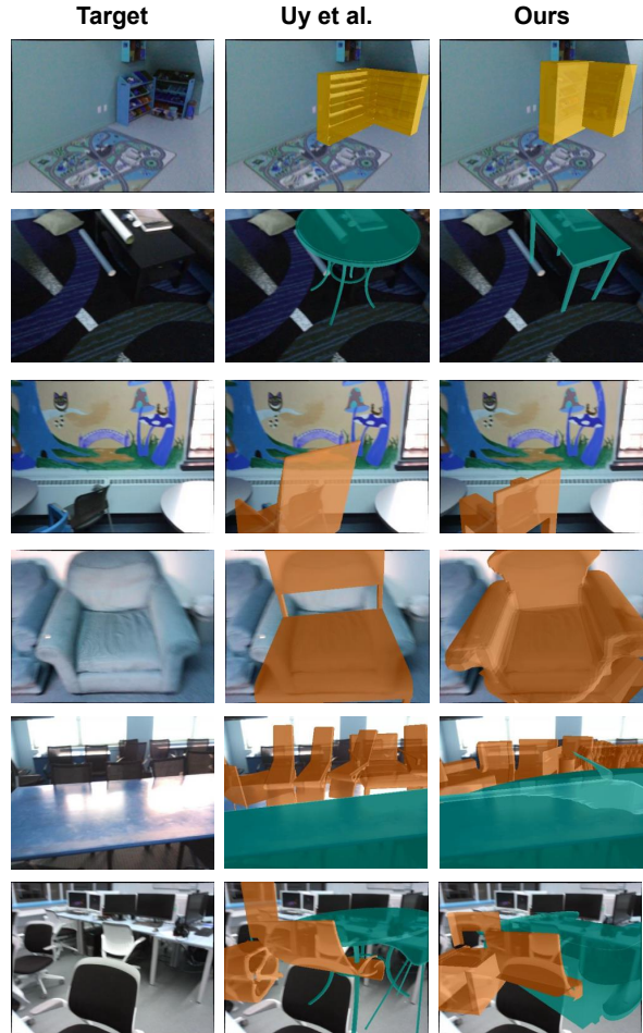
Figure 8. Qualitative results on Scan2CAD [2] dataset with only RGB input. U-RED consistently outperforms state-of-the-art Uy et al. [47].
