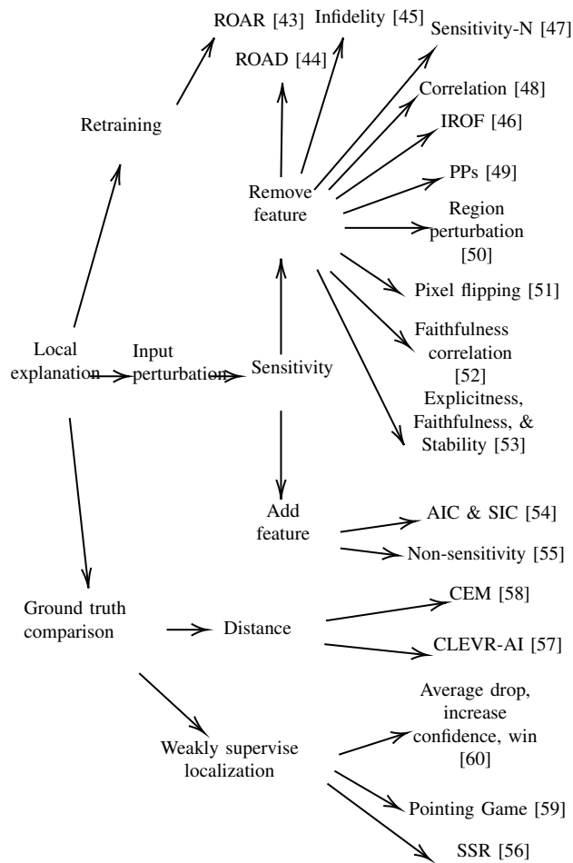
Fig. 4. Proposed taxonomy based the methodologies of the explainability evaluation
