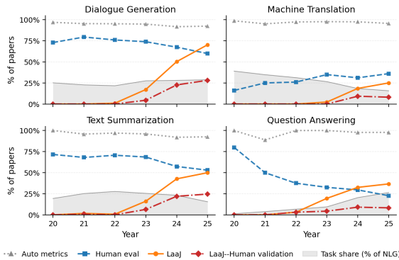
Figure 3: Per-task evaluation method adoption (%) of top-four NLG tasks per year. The filled area shows that task’s share of all NLG papers each year.
