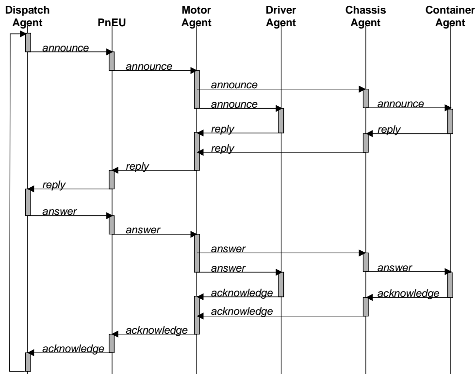
Figure 6: The Interaction Diagram of Internal Agents of a TELETRUCK System
