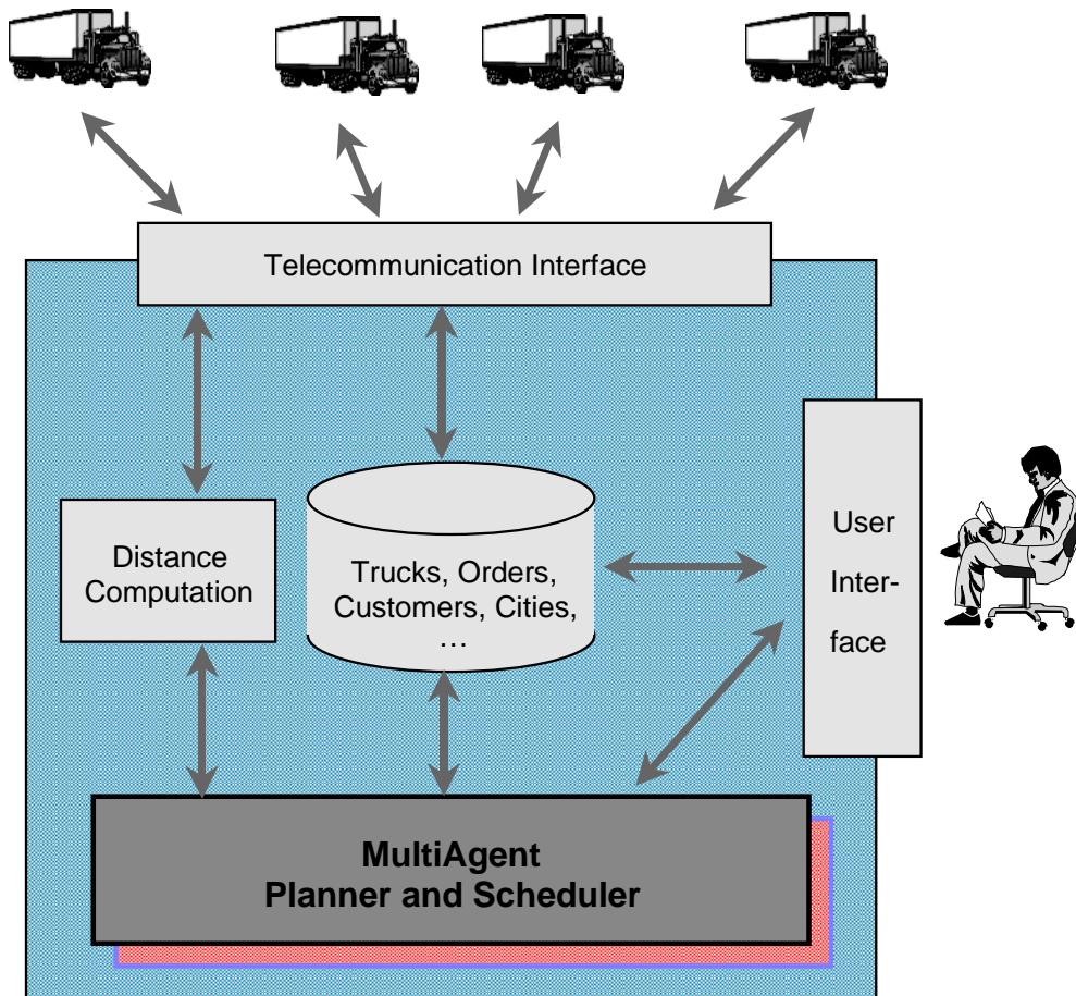
Figure 7: The TELETRUCK-FM Architecture
