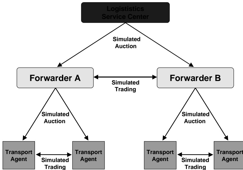
Figure 5: The Holonic Agent Hierarchy of the TELETRUCK Network
