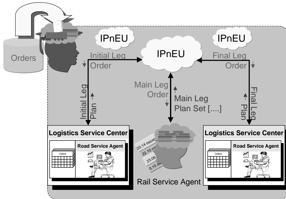
Figure 2: IPnEUs, Road and Rail Service Agents
