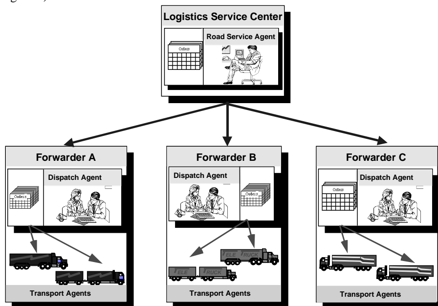
Figure 3: Road Service, Dispatch, and Transport Agents
