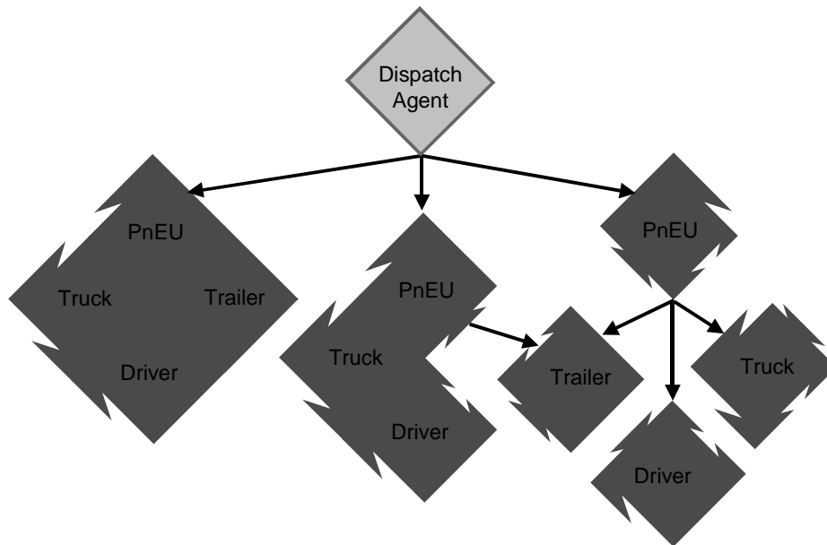
Figure 4: Dispatch Agent and Transport Holons with Component Agents
