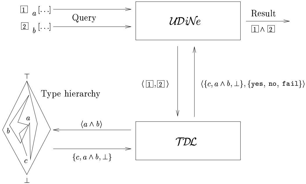
Figure 2.6: Interface between TDL and UDiNe . Depending on the type hierarchy and the type of \boxed{1} and \boxed{2} , TDL either returns c ( c is definitely the GLB of a and b ) or a \wedge b (open-world reasoning) resp. \perp (closed-world reasoning) if there doesn't exist a single type which is equal to the GLB of a and b . In addition, TDL determines whether UDiNe must carry out feature term unification ( yes ) or not ( no ), i.e., the return type contains all the information one needs to work on properly ( fail signals a global unification failure).
