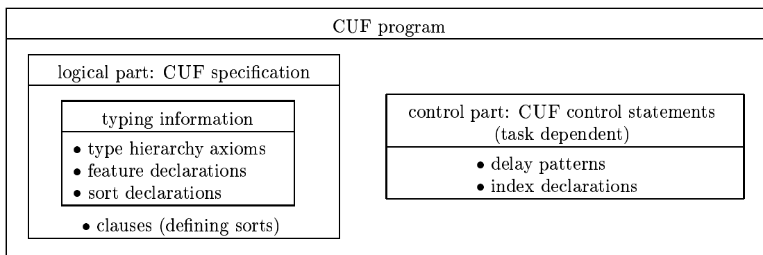
Figure 2.4: Parts of a CUF Program
