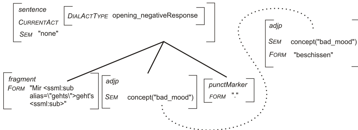
Figure 11: SOCIALITE templates for “Mir geht’s” (“I feel...”) and “beschissen” (“all fucked up”).
