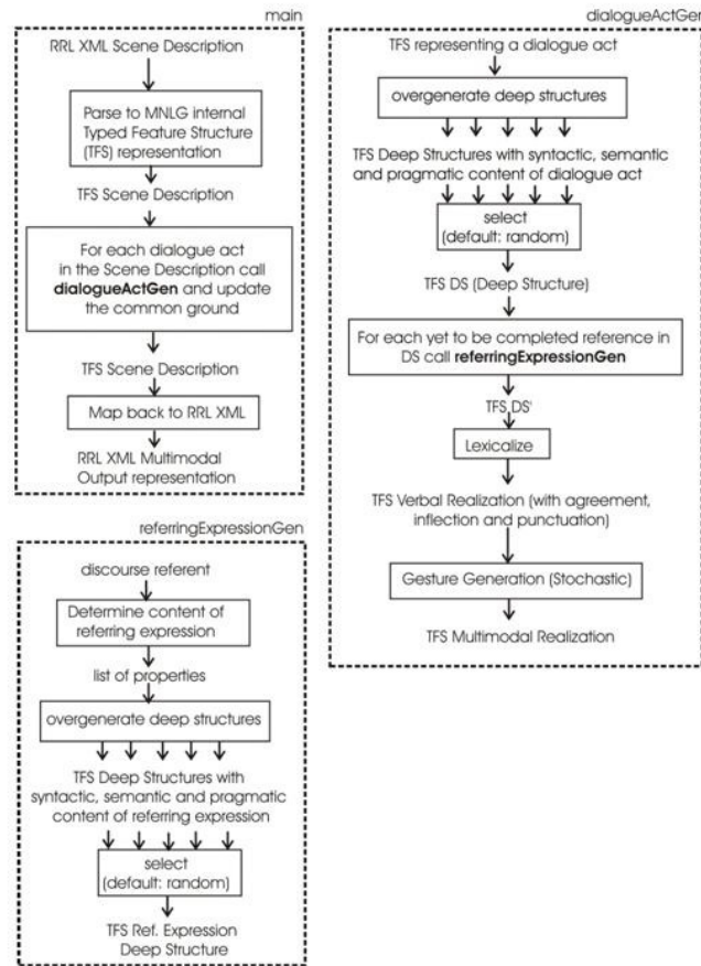
Figure 9: Schematic representation of MNLG architecture
