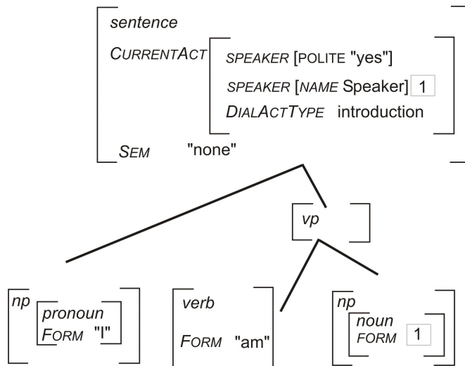
Figure 10: Template for "I am NP"
