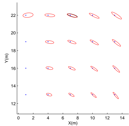
(f) A close look at the estimate of the some features at the lower-left corner of the map (e): dots are true feature positions, 2\sigma covariance ellipses are from I-SLSJF
