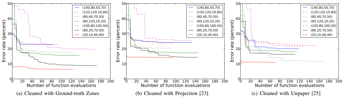
Fig. 2. Result of optimizing parameters of the X-Y Cut algorithm on UW-III dataset and its cleanup versions. Different curves correspond to different starting points (with values given in the legend) of the Simplex optimization algorithm.
