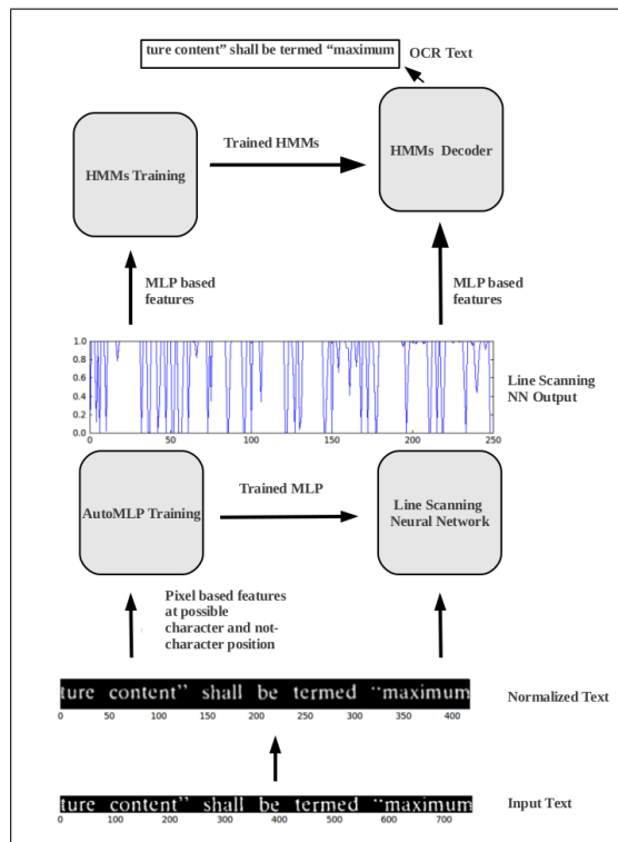
Figure 1. Line scanning neural network architecture.
