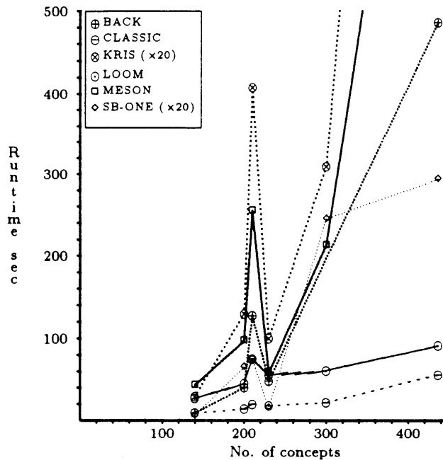
Figure 1: Runtime performance on real KBs
