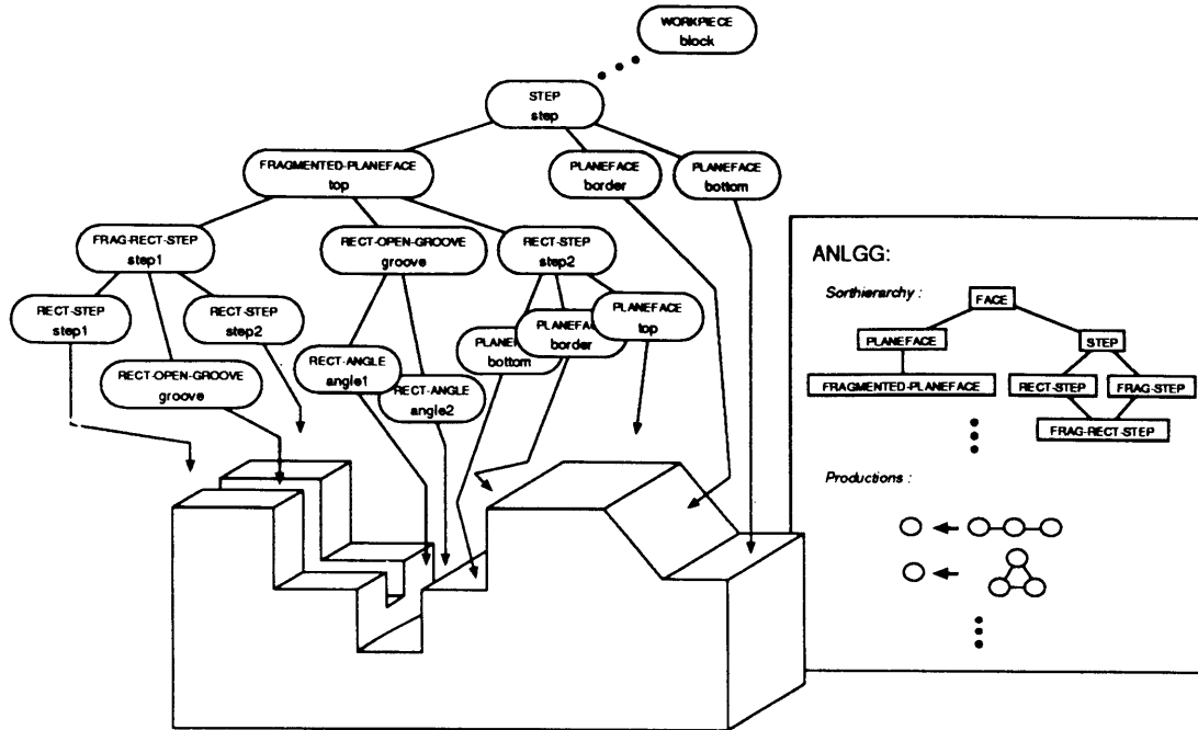
Figure 5: A workpiece and a part of the feature tree generated by the parser
