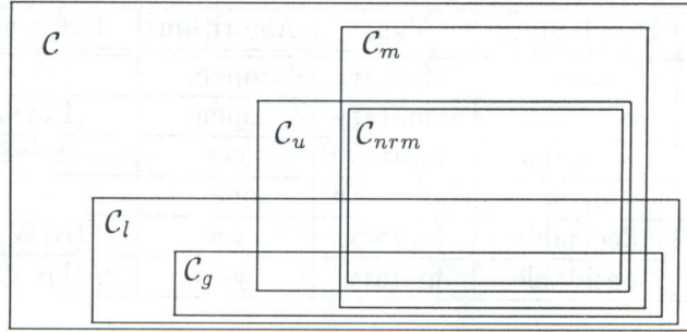
Figure 10: The relation between the classes \mathcal{C} , \mathcal{C}_l , \mathcal{C}_g , \mathcal{C}_m , \mathcal{C}_{nrm} , and \mathcal{C}_u .
