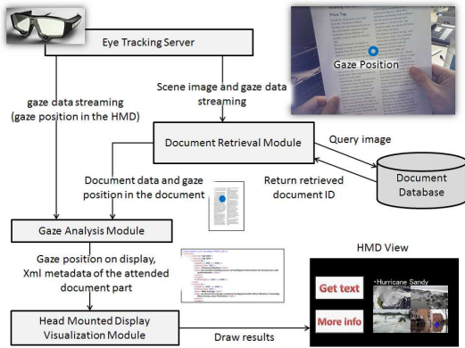
Fig. 2. The workflow image.
