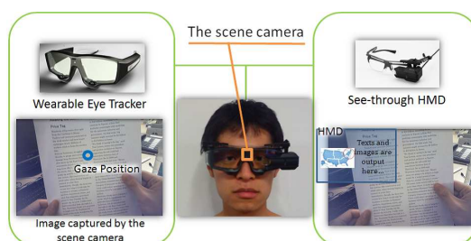
Fig. 1. We combine a wearable eye tracker and a see-through head mounted display. The scene image is captured by the scene camera of the eye tracker (integrated into the center of the frame).
