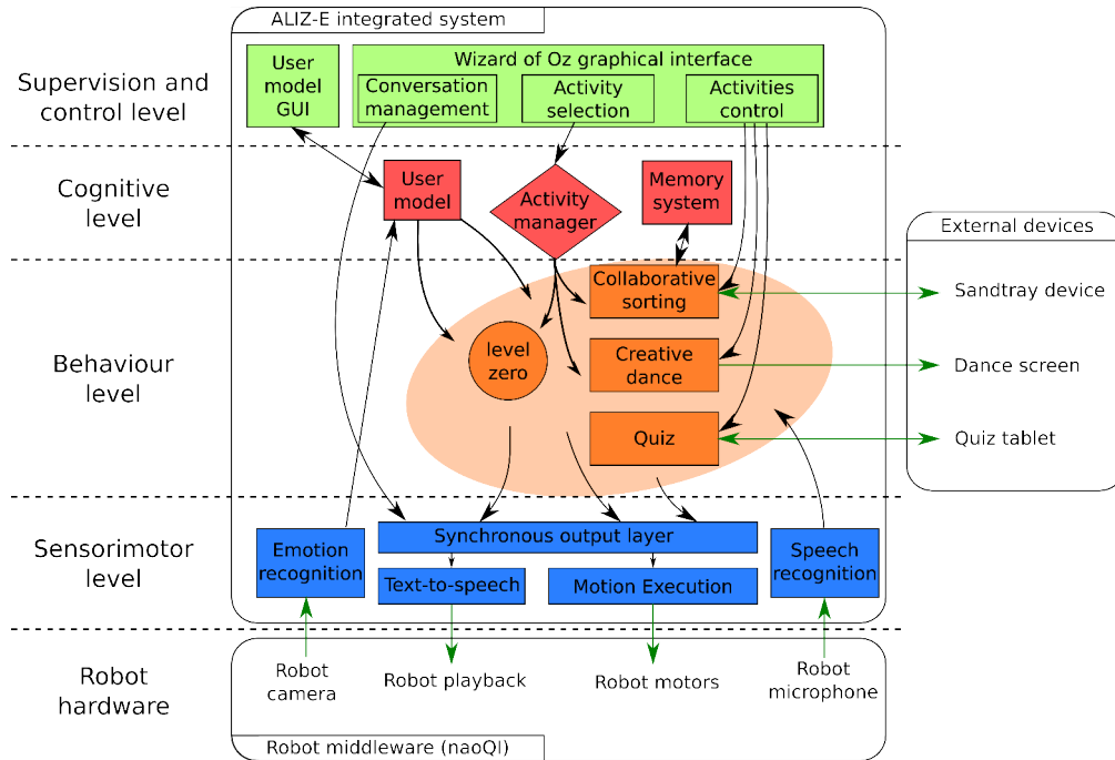
Figure 3. : Schematic description of the integrated system architecture. Black arrows depict Urbi messages exchanges (see section 4.4), while green arrows show interaction with the robot middleware or external devices. The low-level motor components are shown in blue, the activities that determine the robot behaviour in orange, the intermediate cognitive structures (memory, behaviour selection, etc.) in red, and the top-level wizard-based control system in green.
