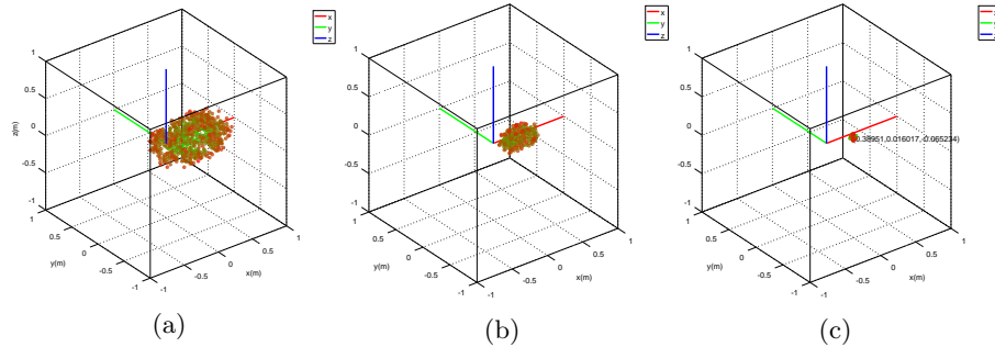
Fig. 5: 3-D translational convergence to (0.40, 0.025, -0.07) m
