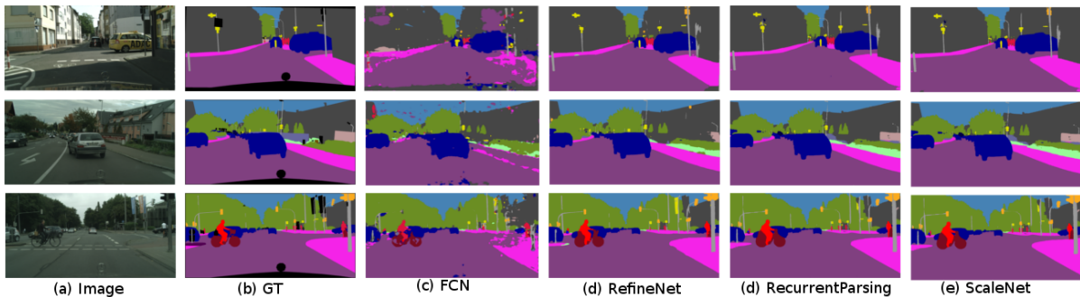
Figure 3: Qualitative evaluation of FCN-8s (Long et al., 2015b), RefineNet (Lin et al., 2016a), RecurrentParsing (Kong and Fowlkes, 2017) and ScaleNet (our) for benchmark dataset Cityscapes (validation set).
