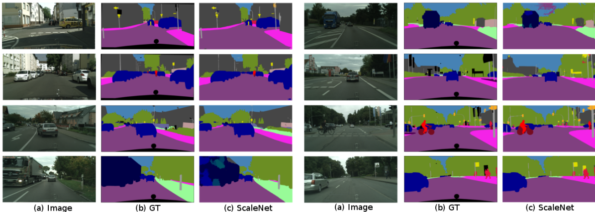
Figure 1: Qualitative evaluation of ScaleNet (ours) compared to the ground truth of the benchmark dataset Cityscapes (validation set).
