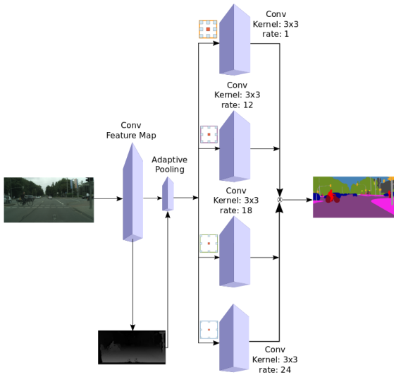
Figure 2: Architecture of the desired model is shown. This model generates depth as the intermediate result, which is used for adaptive pooling.
