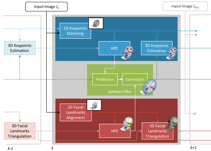
Fig. 1: Proposed HPE pipeline, from Keypoints (blue) and Facial Landmarks (red).
