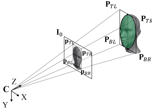
Fig. 5: Initialization of the ellipsoid. Source: [11]
